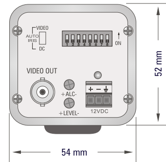
CCD480-AD Back Side View
